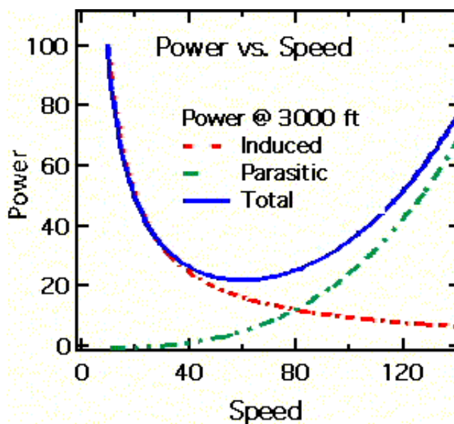
Fig 11 Power requirements versus speed.
