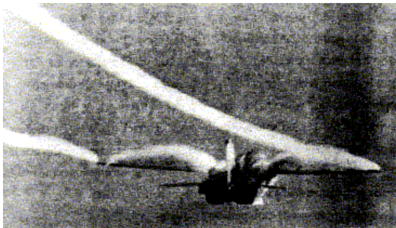
Fig 15 Condensation showing the distribution of lift along a wing. The wingtip vortices are also seen.
